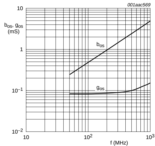
Fig 16. Amplifier A: output admittance as a function of frequency; typical values
